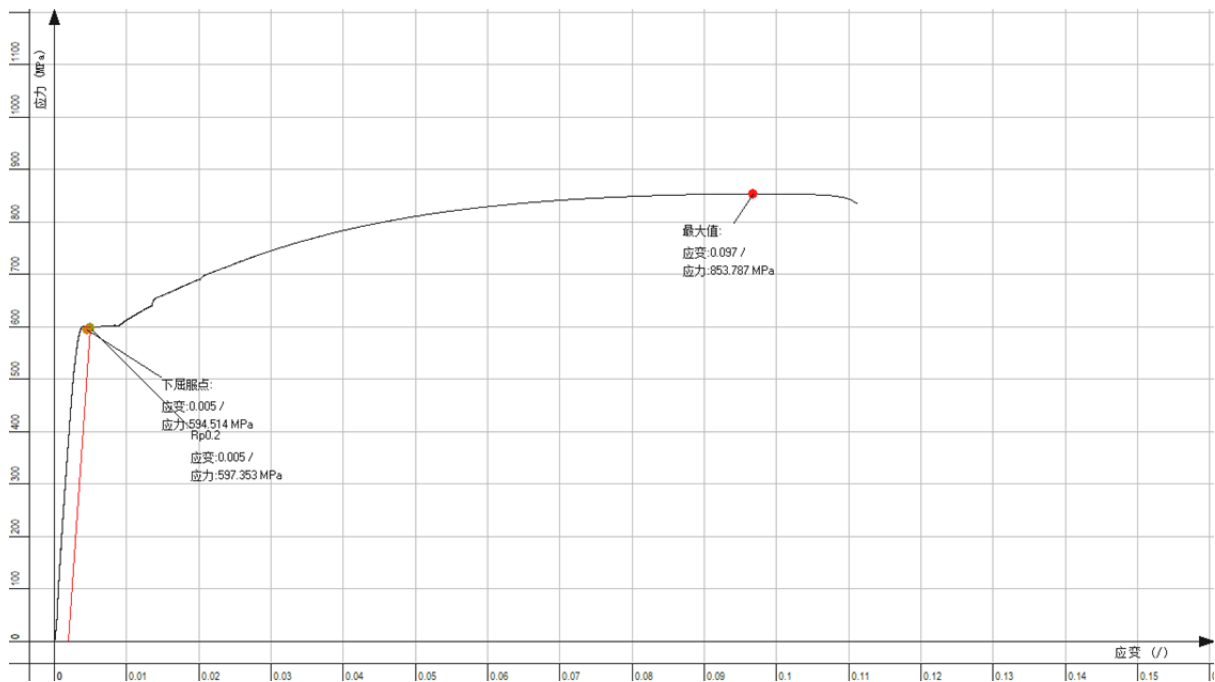
Stress-strain curve
