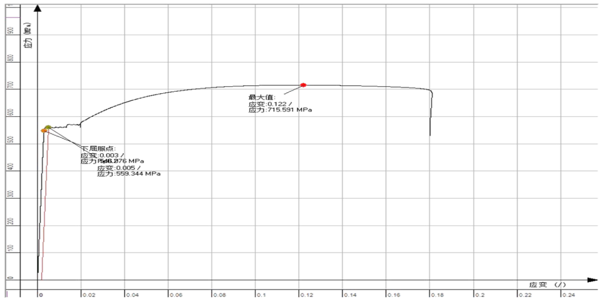
Tensile Test Curve Chart
